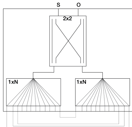
Internal Switch Diagram
